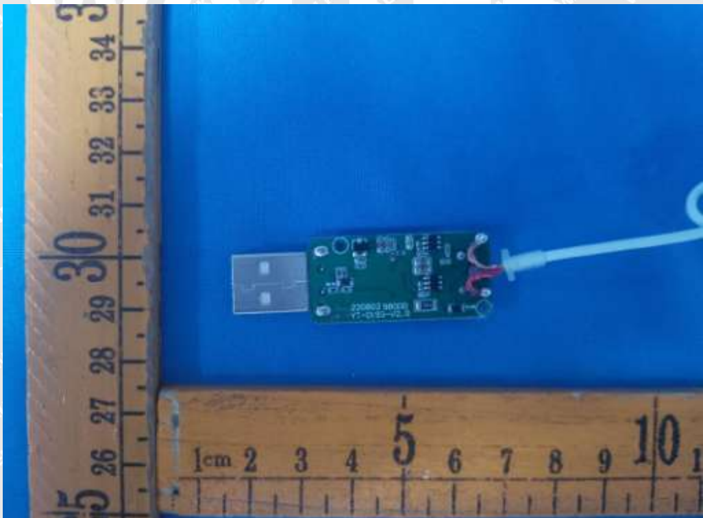
Photo 16 PCB view
